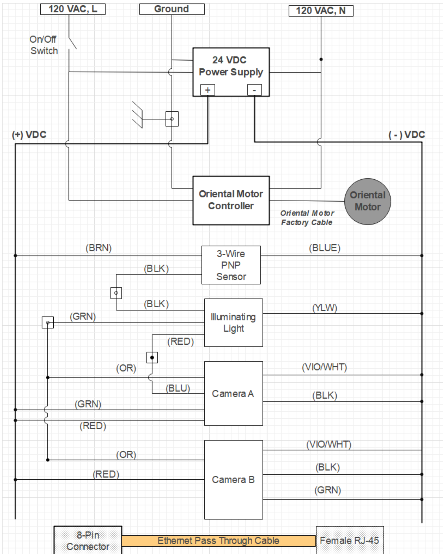
Zebra Demo Units Schematic March 2022
